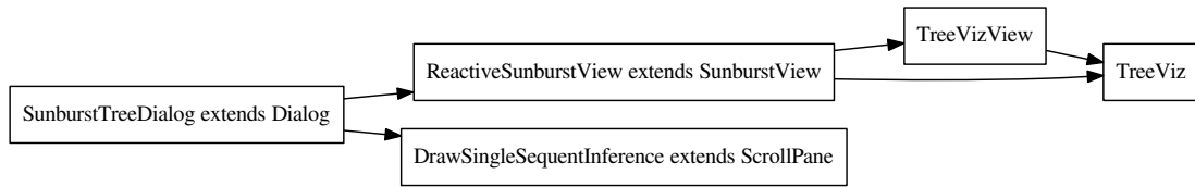
Figure 7: Architecture of SUNBURSTTREEIALOG
